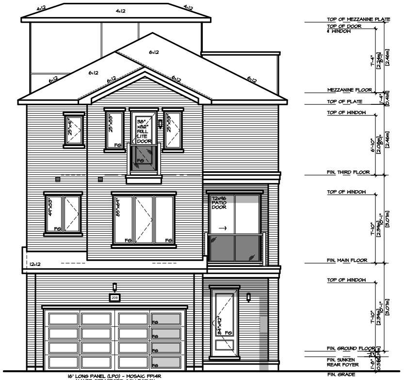
REAR ELEVATION 'MO' MODERN
