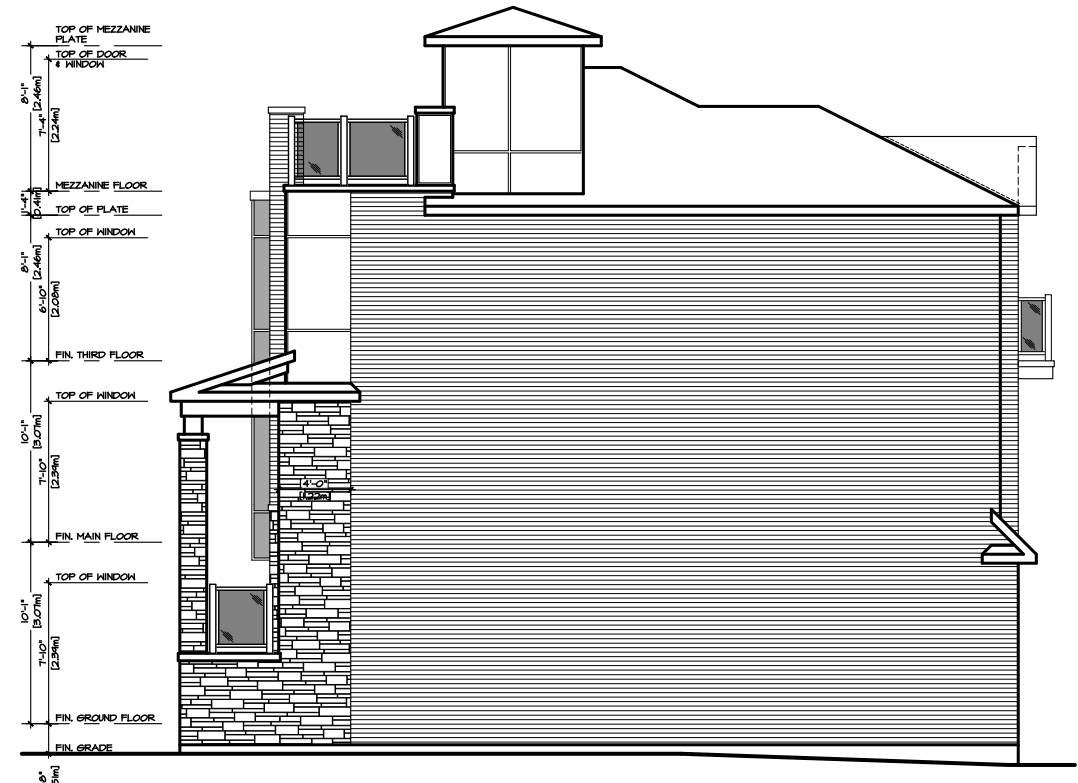
RIGHT SIDE ELEVATION 'MO' MODERN
