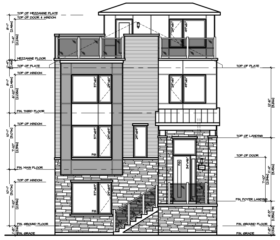
FRONT ELEVATION 'MO' MODERN
