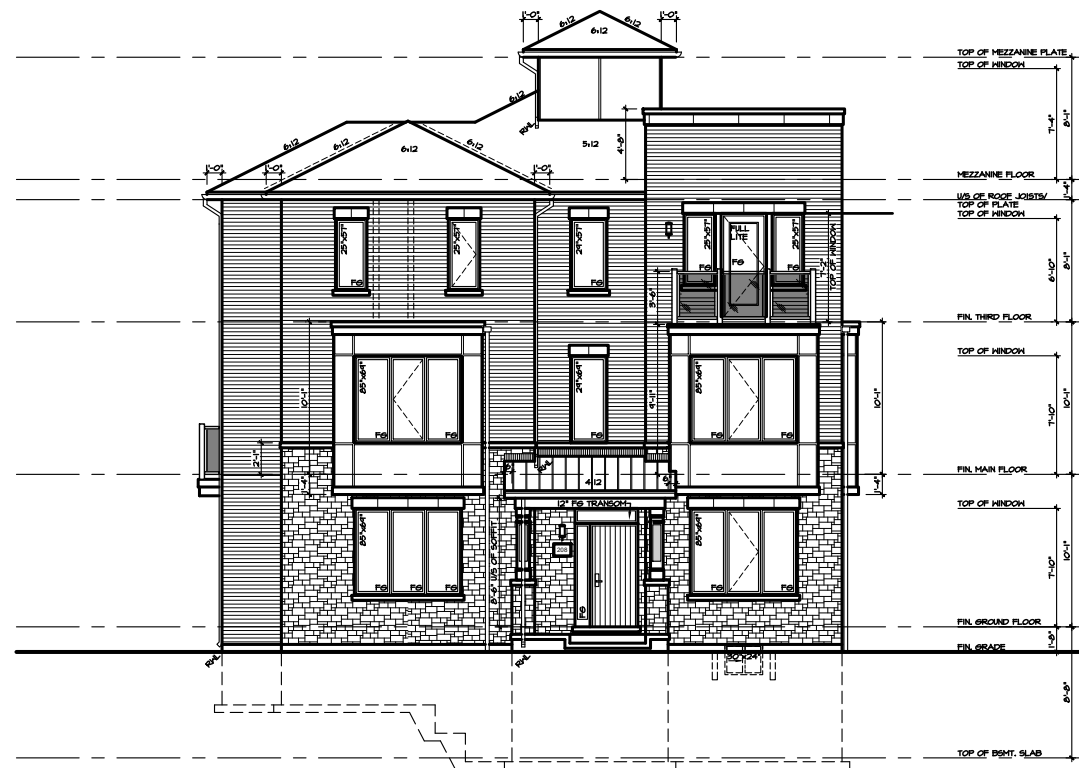
① UNIT GR1E THE MERLOT CORNER ELEV. TA
