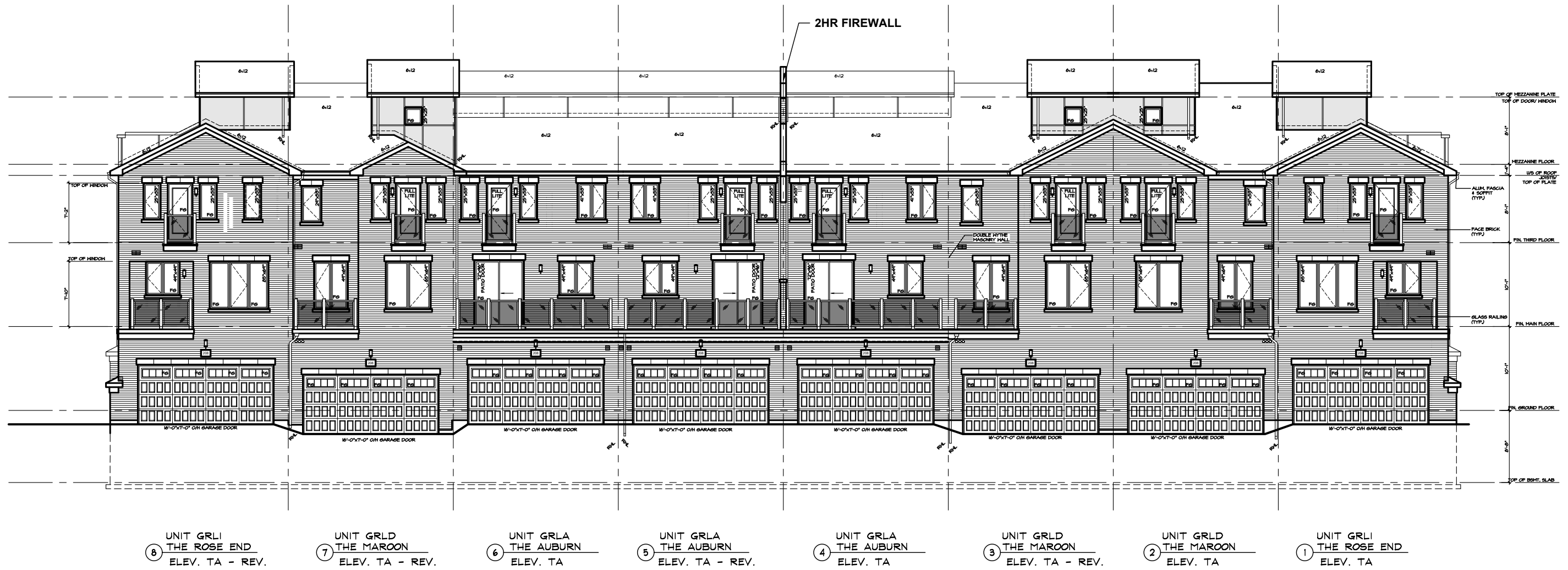
REAR ELEVATION ELEVATION TA REAR LANE TOWNS BLOCK 30
