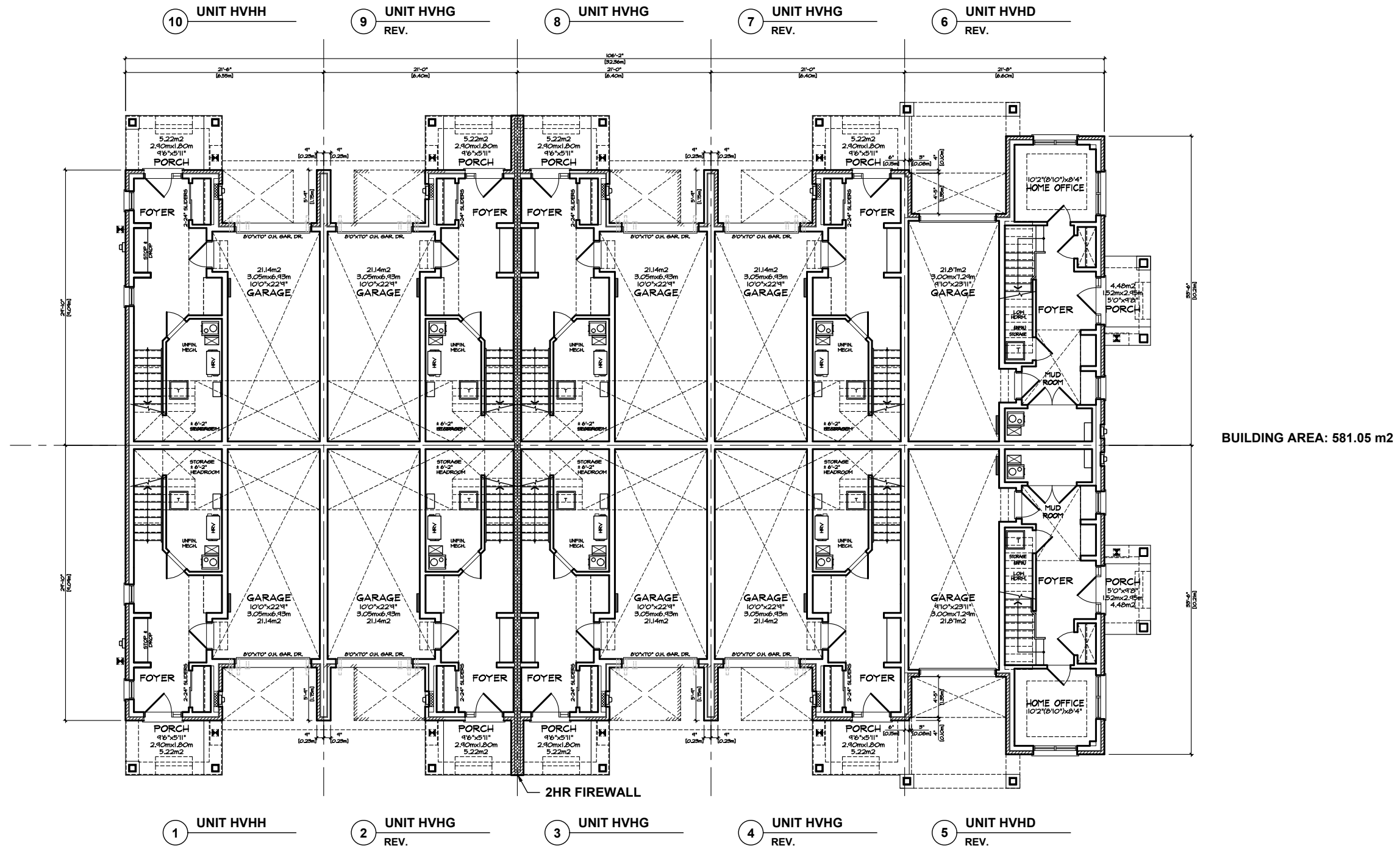
GROUND FLOOR PLAN 'TA' VILLAGE HOMES BLOCK 37
