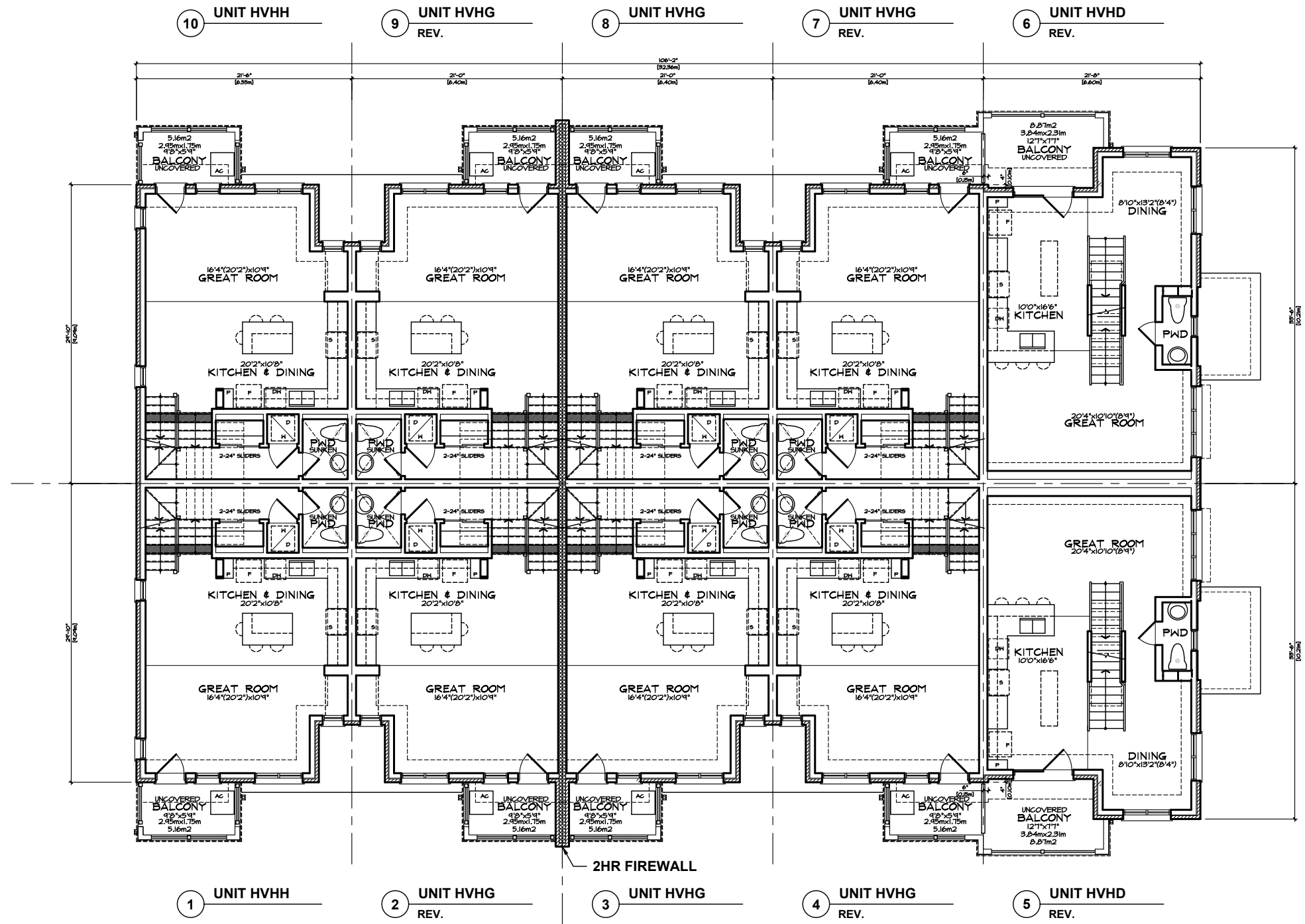
MAIN FLOOR PLAN 'TA' VILLAGE HOMES BLOCK 37
