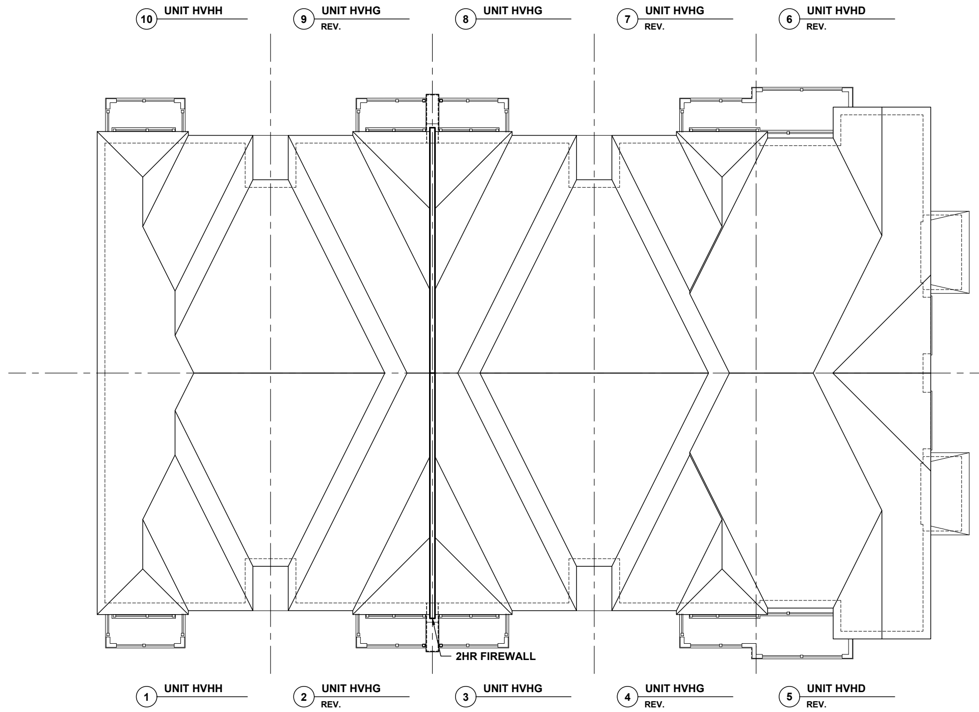
ROOF PLAN 'TA' VILLAGE HOMES BLOCK 37
