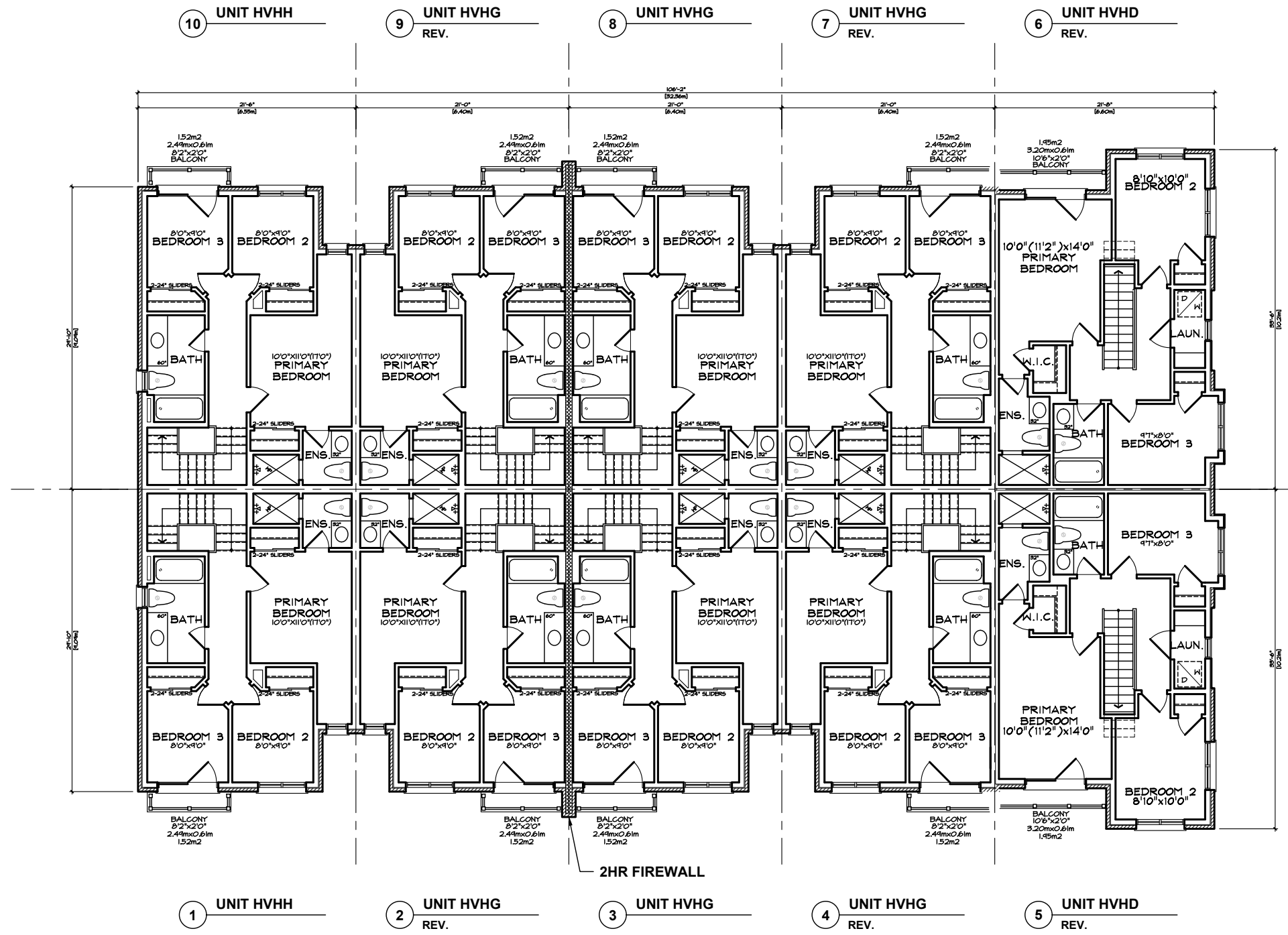
THIRD FLOOR PLAN 'TA' VILLAGE HOMES BLOCK 37
