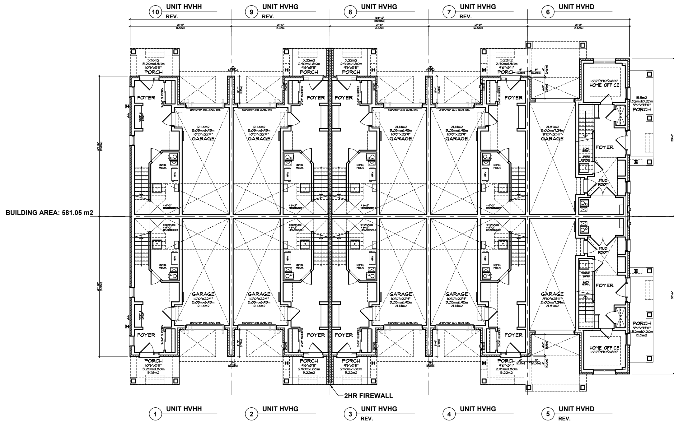
GROUND FLOOR PLAN 'FM' VILLAGE HOMES BLOCK 38
