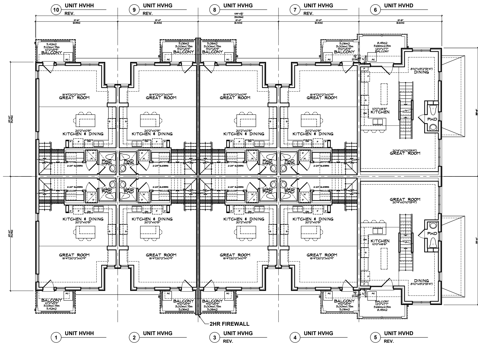
MAIN FLOOR PLAN 'FM' VILLAGE HOMES BLOCK 38
