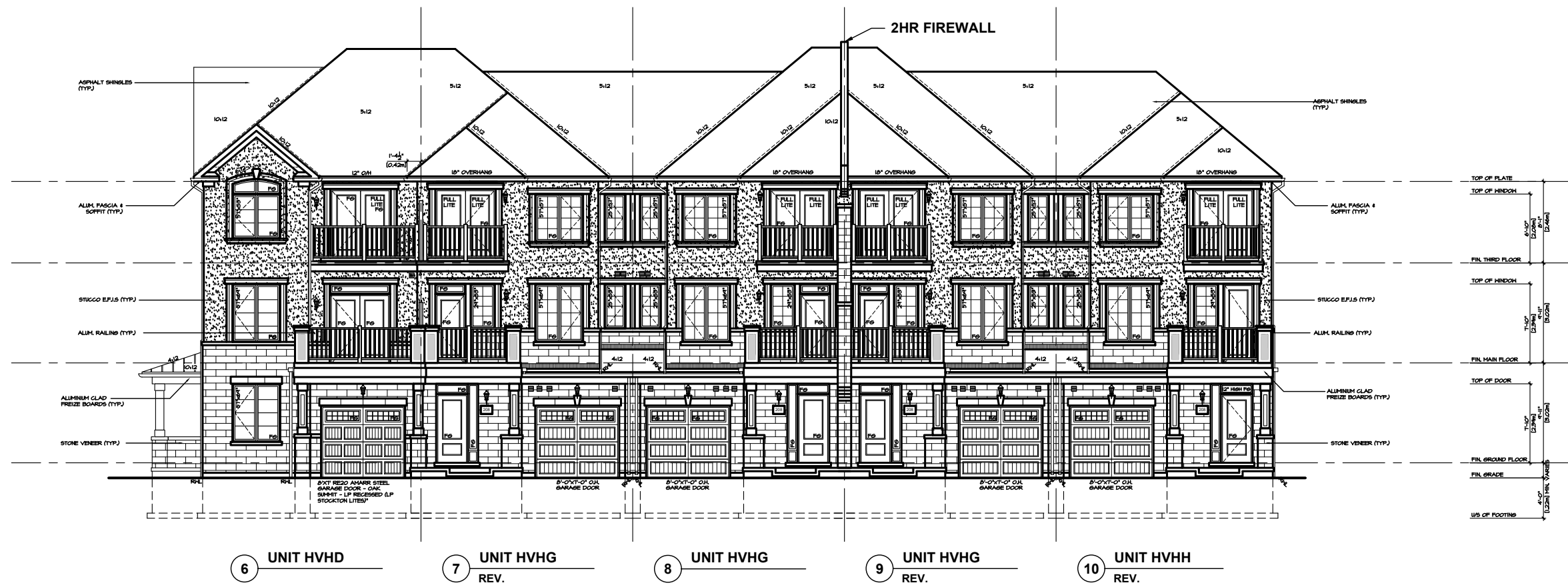
NORTH ELEVATION 'FM' VILLAGE HOMES BLOCK 38
