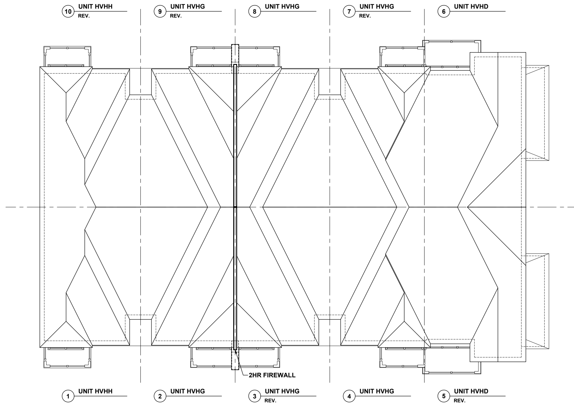
ROOF PLAN 'FM' VILLAGE HOMES BLOCK 38
