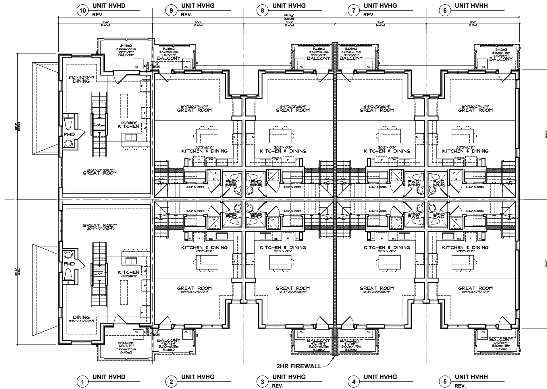
MAIN FLOOR PLAN 'FM' VILLAGE HOMES BLOCK 39
