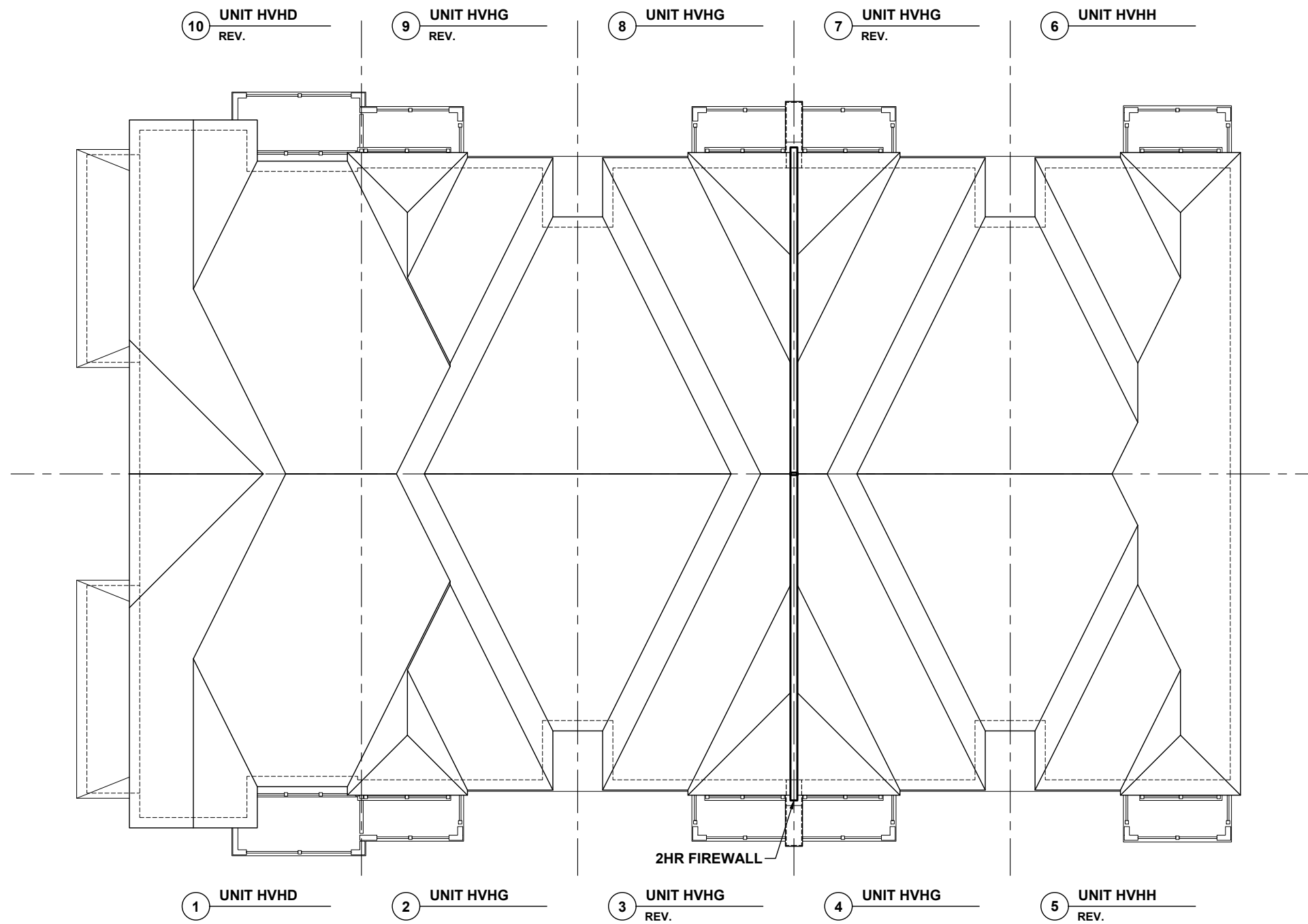
ROOF PLAN 'FM' VILLAGE HOMES BLOCK 39
