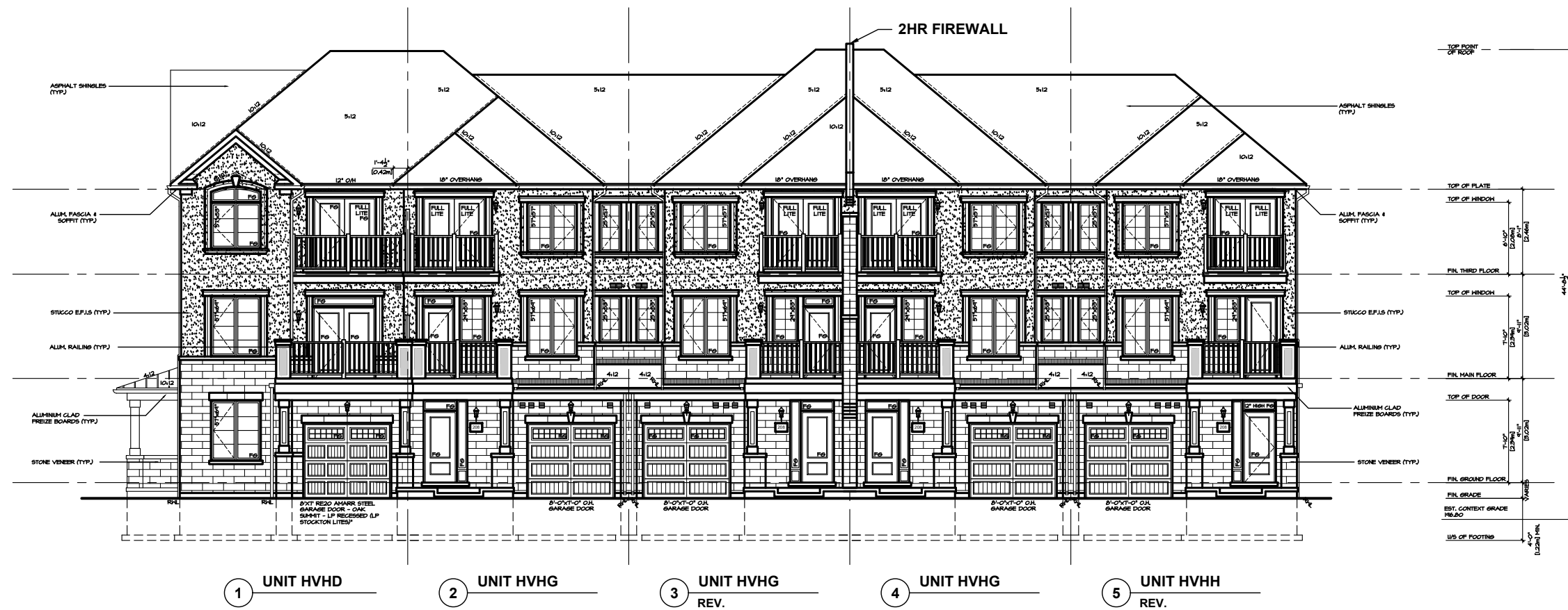
SOUTH ELEVATION 'FM' VILLAGE HOMES BLOCK 39
