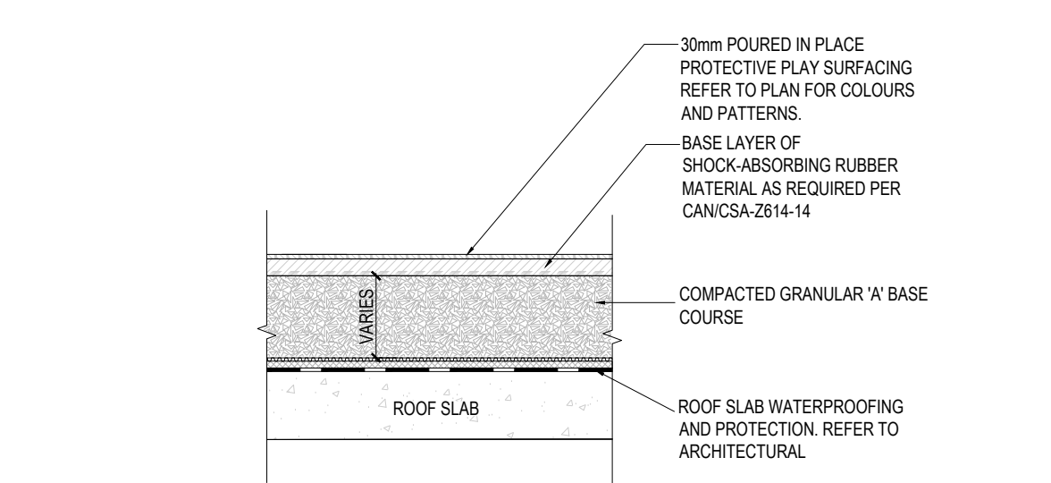
4 PROTECTIVE PLAY SURFACE 1:20
