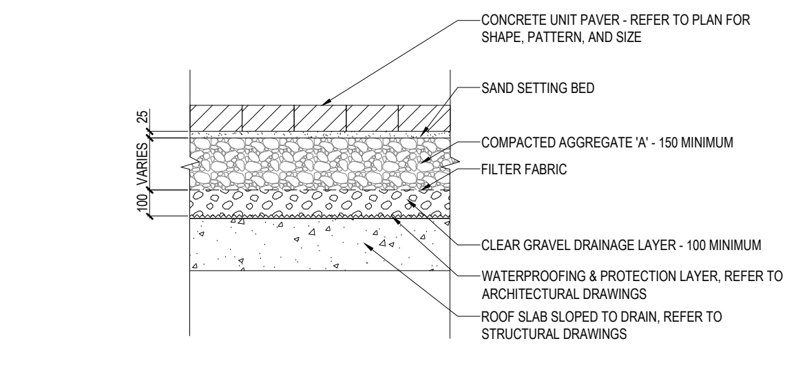
2 PEDESTRIAN UNIT PAVERS ON ROOF SLAB 1:20
