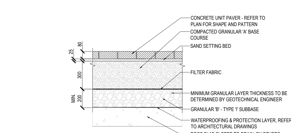
3 HEAVY DUTY UNIT PAVER ON SLAB SCALE=1:20
