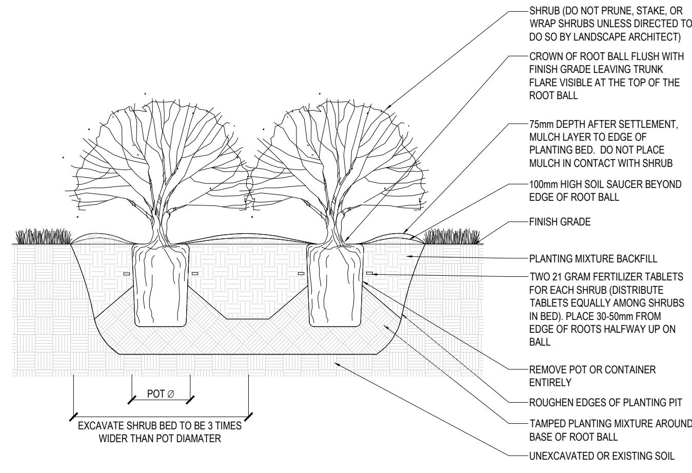
6 POTTED SHRUB BED PLANTING DETAIL N.T.S.
