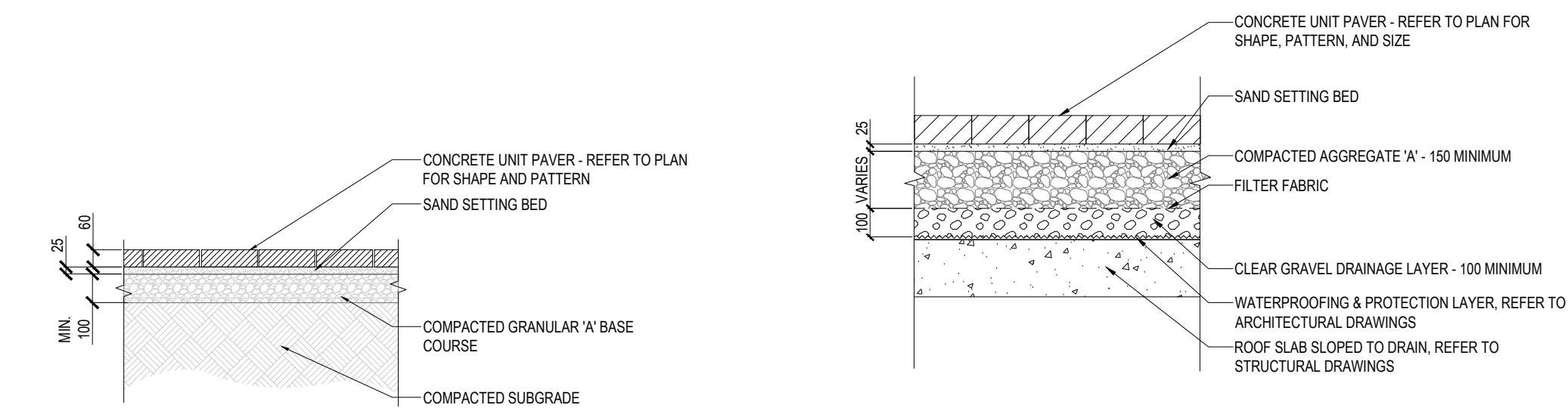
1 ON GRADE UNIT PAVER SCALE=1:20
