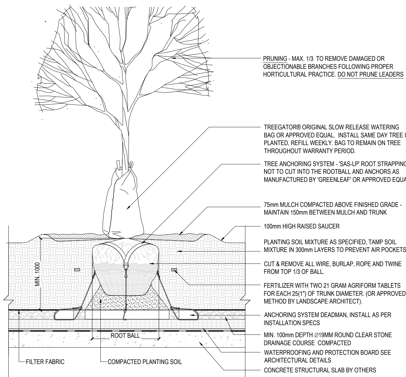
5 DECIDUOUS TREE PLANTING ON SLAB 1:25
