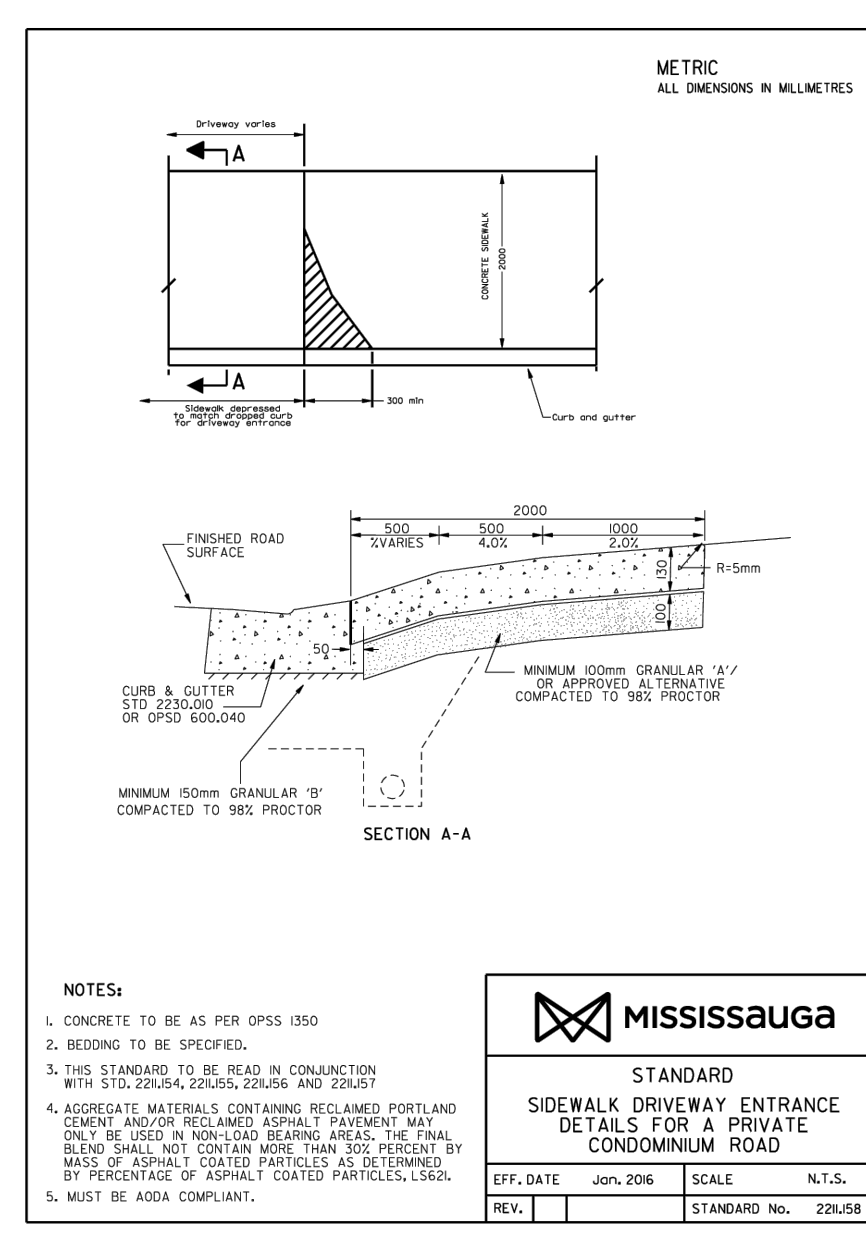
3 DRIVEWAY ENTRANCE N.T.S.
