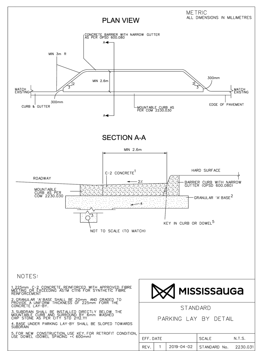
6 LAY BY PARKING N.T.S.
