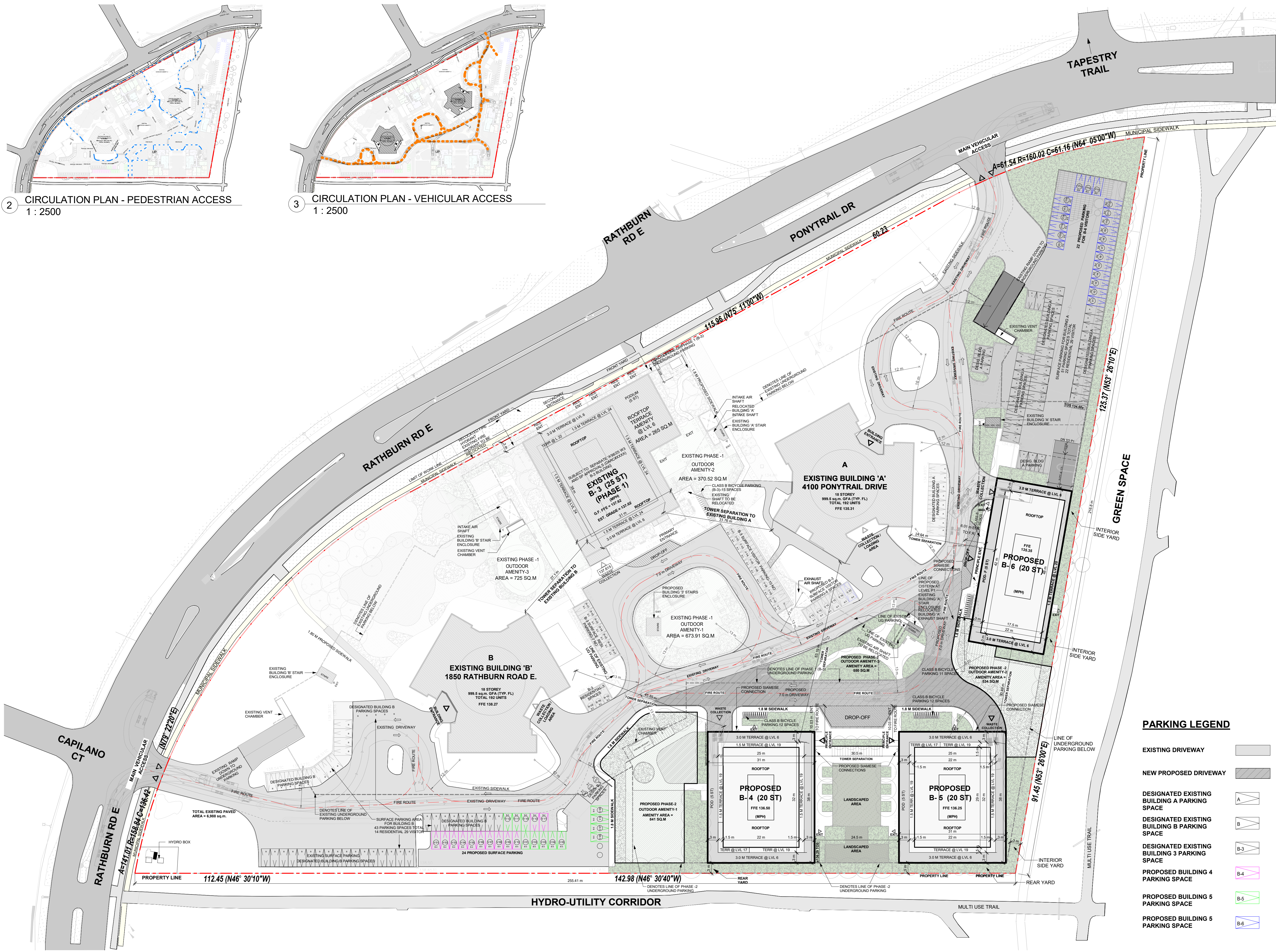
1 PHASE 2 - OVERALL SITE PLAN 1 : 500
