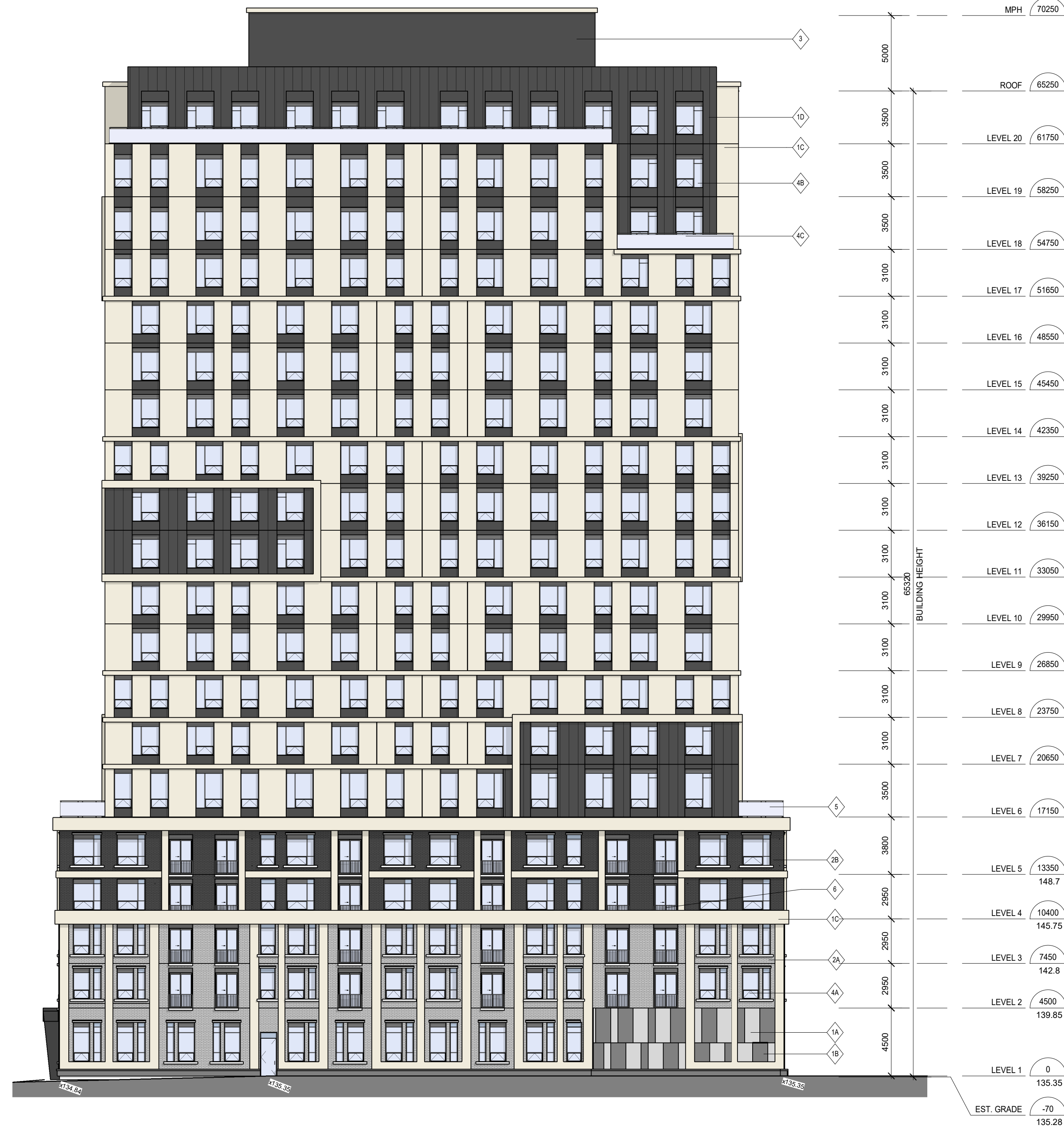
1 EAST ELEVATION 1 : 200
