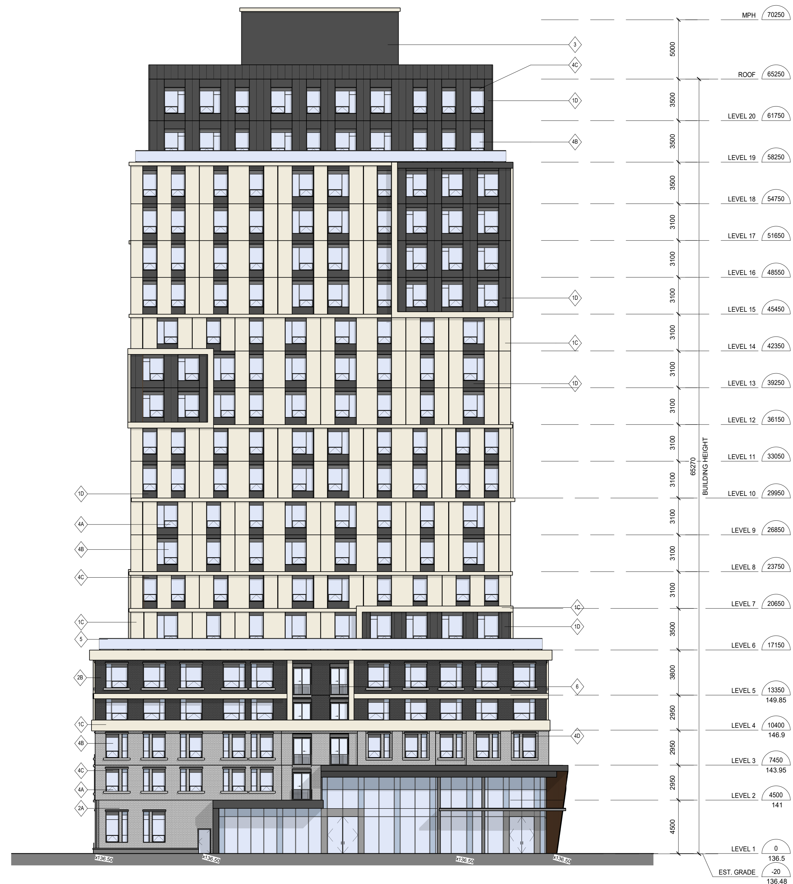
1 EAST ELEVATION 1 : 200
