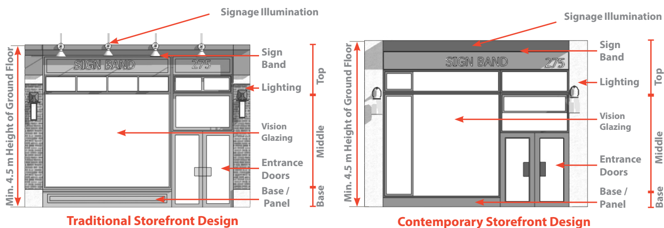
Figure 20: Storefronts can incorporate a variety of styles and character to animate the street edge. When well executed, they contribute to the identity of the street and make retail and commercial frontages inviting and accessible to pedestrians
