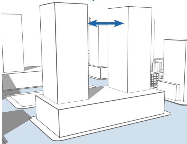
Figure 47: Tower Separation: Spacing towers with minimum separation will minimize collective shade and sunlight impacts of closely-spaced towers on streets, parks and adjacent residential buildings. This will also achieve increased access to sky views and natural lighting as well as increased privacy. The spacing between point towers will be a minimum of 30.0 m.
