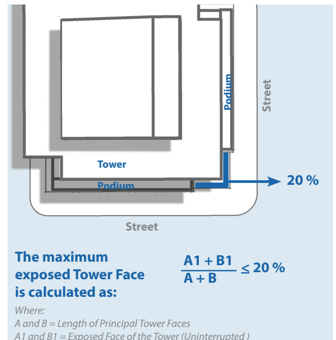
Figure 49: Calculation of uninterrupted tower shafts.
