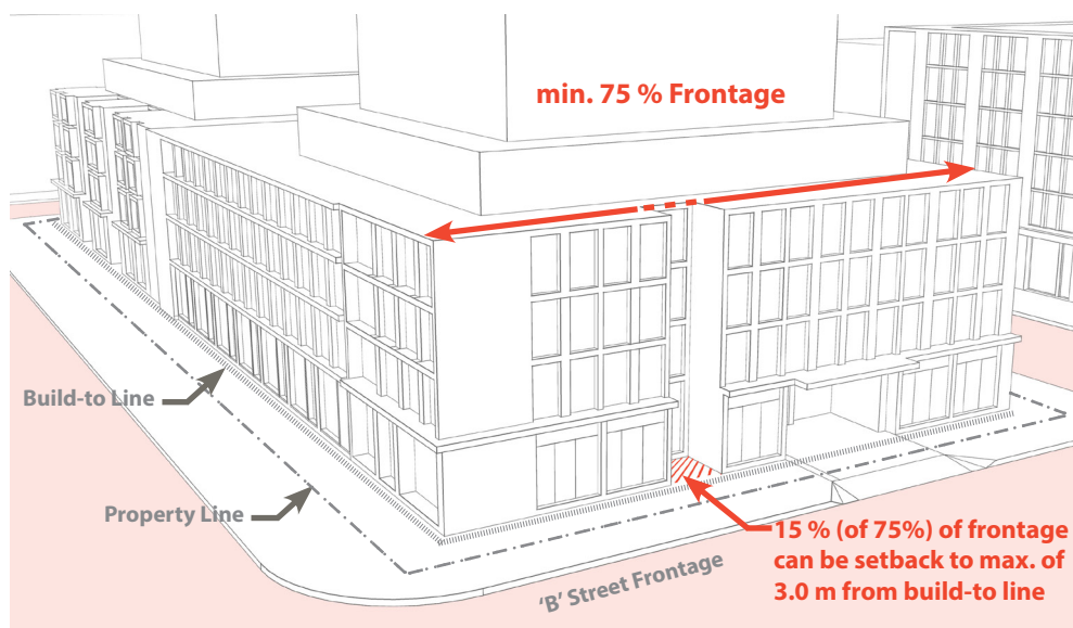
Figure 11: Example of recessed loading on B Street.
