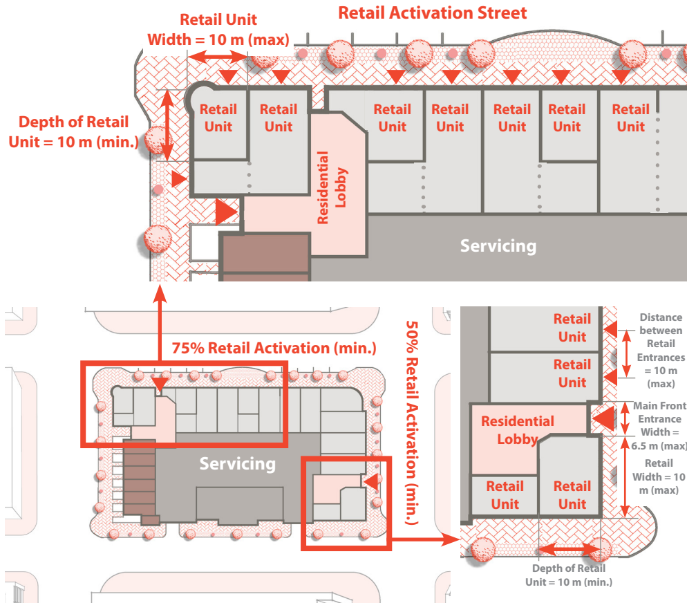
Figure 24: Interior demising walls for retail units can be configured to promote an expression of narrower units and smaller retail spaces along building frontages, opening up beyond to combine units into larger retail spaces.
