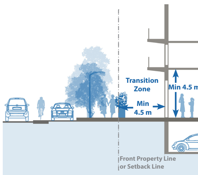
Figure 60: Approach II: Residential uses are located at the same level of the public sidewalk, with individual entrances, but designed for potential conversion to retail and or commercial.
