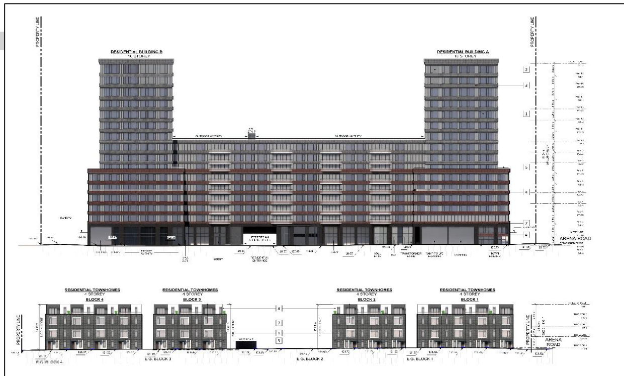
West Elevation (Dundix Road)
